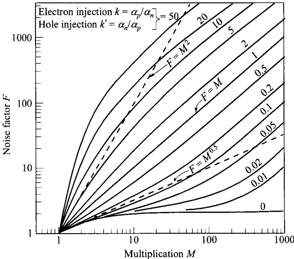
Fig. 13 Theoretical noise factor vs. multiplication, for different ratios of electron and hole ionization coefficients. (After Ref. 20.)
