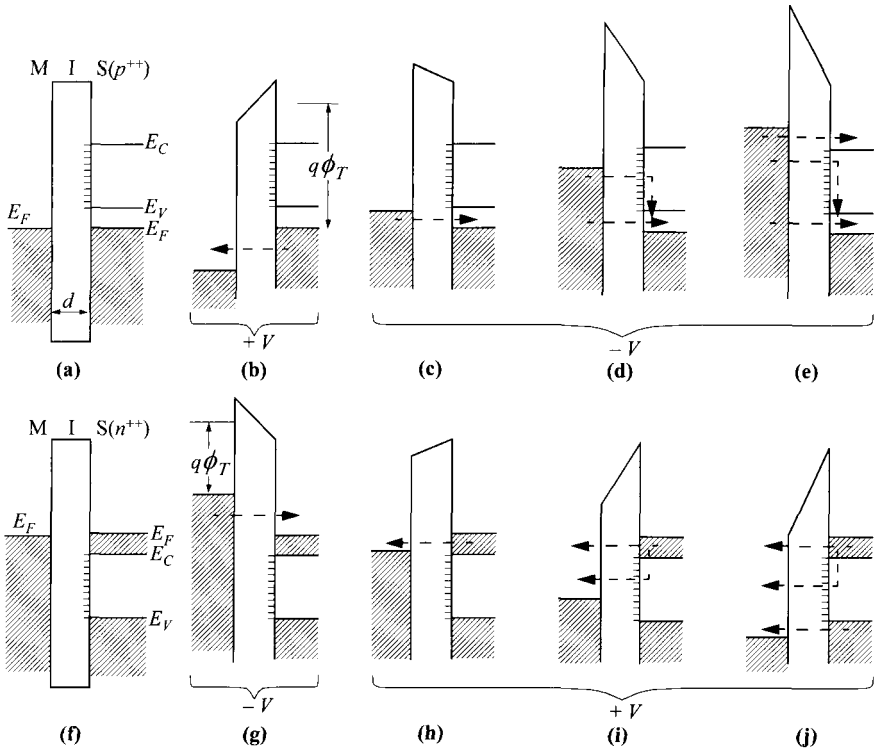
Fig. 23 Simplified band diagrams of MIS tunnel diodes on degenerate substrates, including interface traps. Top and bottom rows are for p^+ - and n^+ -substrates respectively. V is positive bias on the metal. (After Ref. 49.)
